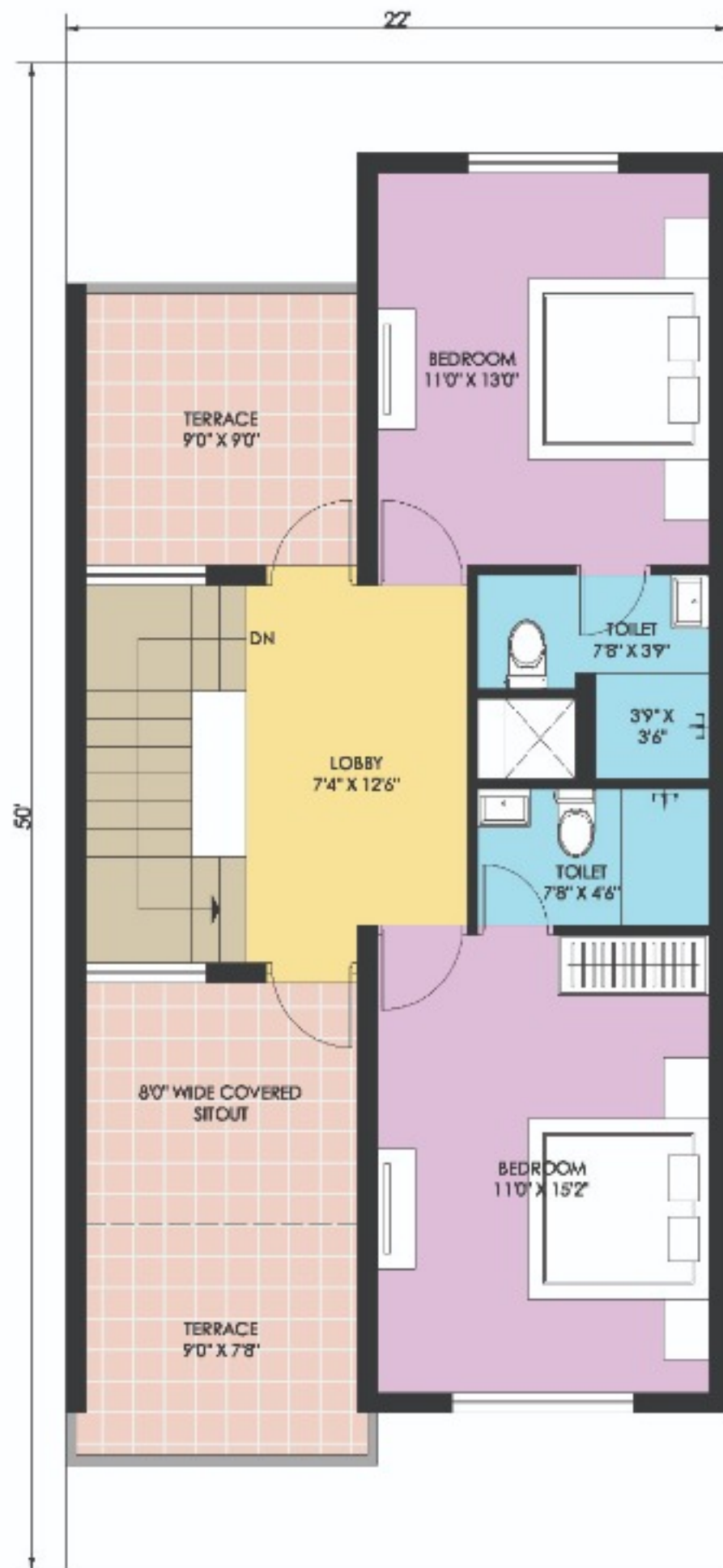
FIRST FLOOR PLAN sbua- 726.0 sq.ft.
