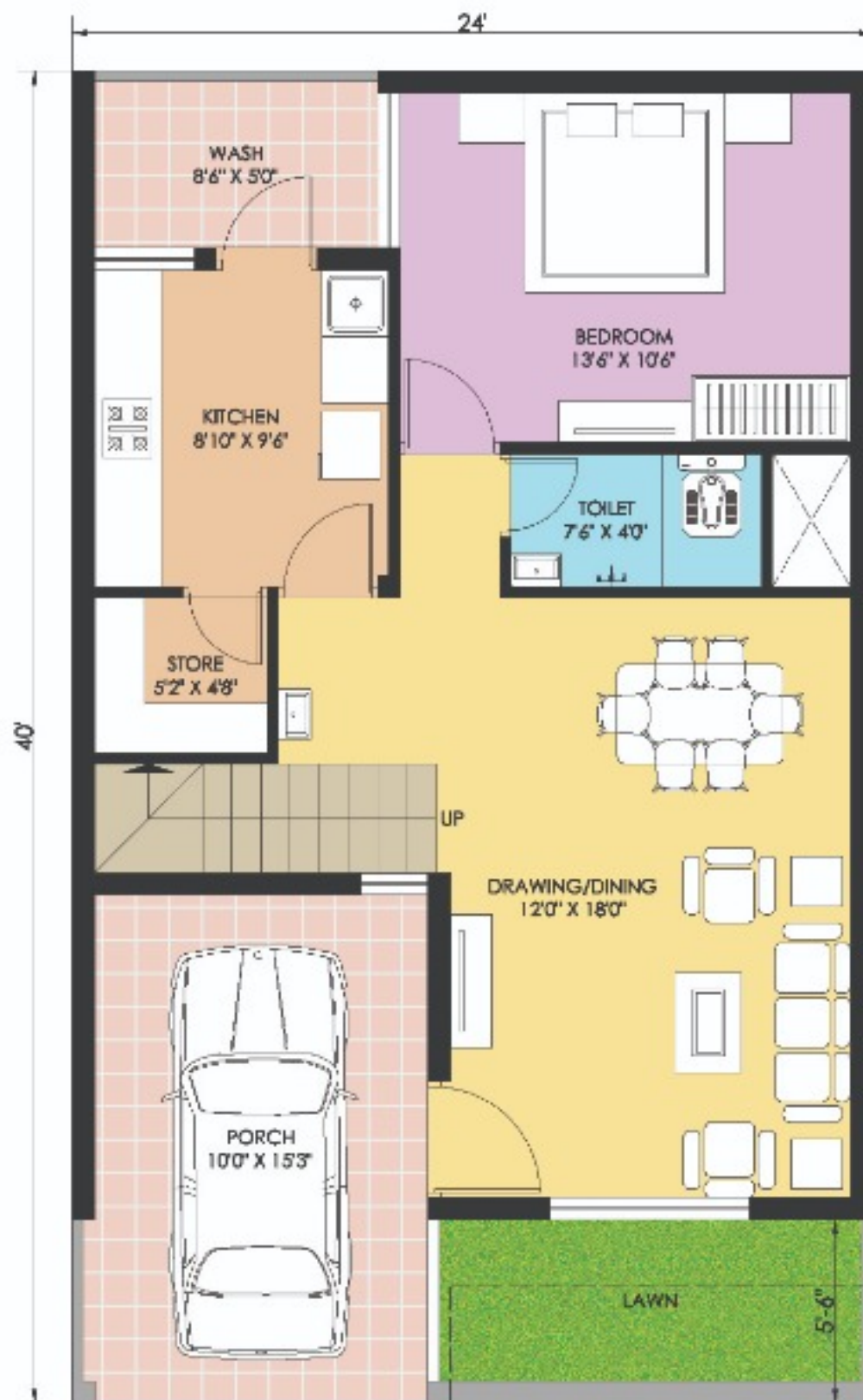
GROUND FLOOR PLAN sbua- 916.0 sq.ft.
