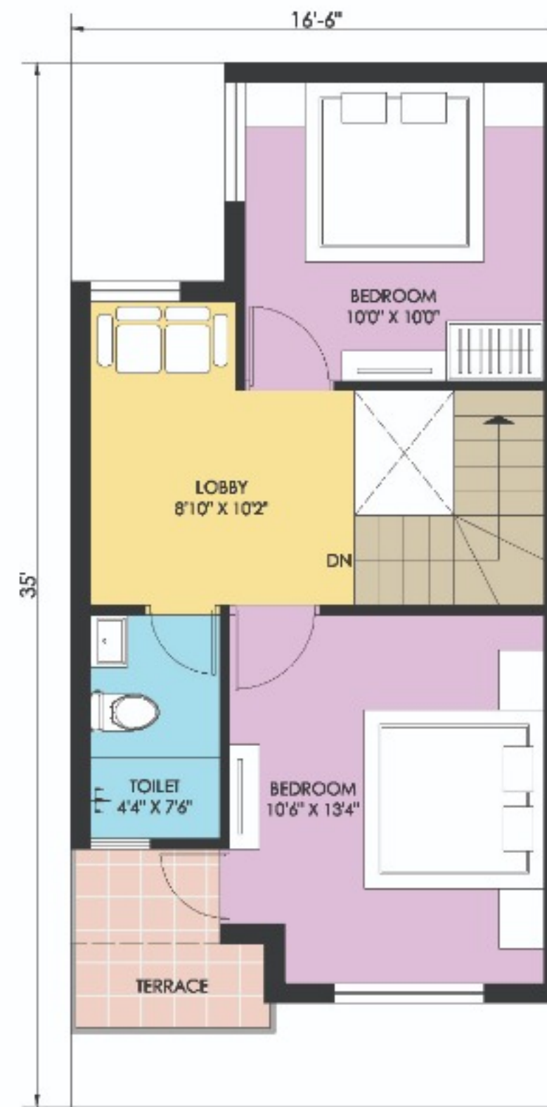
FIRST FLOOR PLAN sbua- 469.0 sq.ft.
