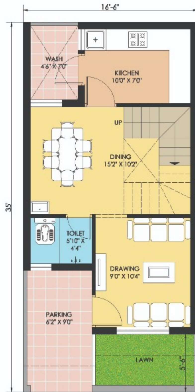
GROUND FLOOR PLAN sbua- 489.0 sq.ft.
